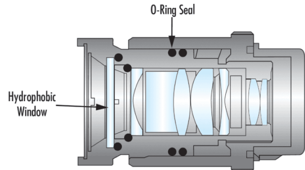
35mm Cw Series Fixed Focal Length Lens
