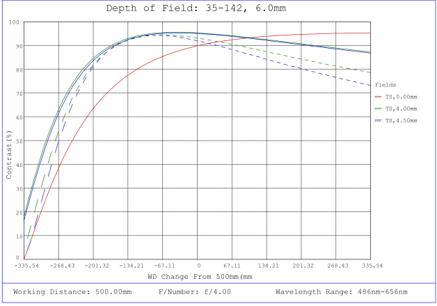
#35-142, 6mm, f/4 Cr Series Fixed Focal Length Lens, Depth of Field Plot, 500mm Working Distance, f4
