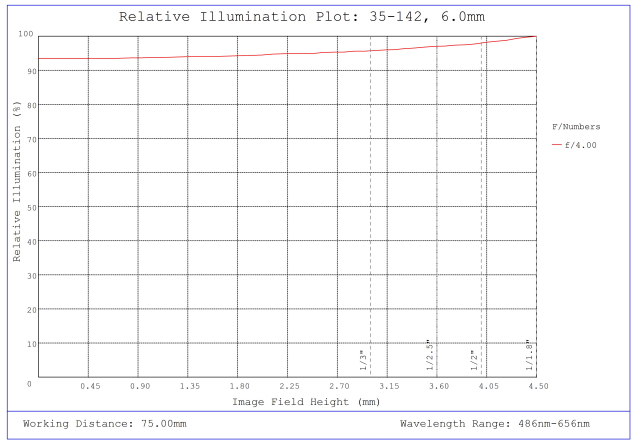
#35-142, 6mm, f/4 Cr Series Fixed Focal Length Lens, Relative Illumination Plot
