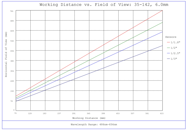
#35-142, 6mm, f/4 Cr Series Fixed Focal Length Lens, Working Distance versus Field of View Plot
