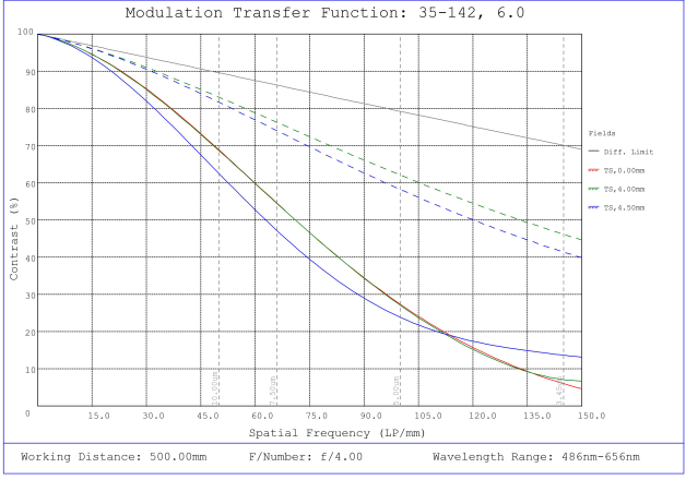
#35-142, 6mm, f/4 Cr Series Fixed Focal Length Lens, Modulated Transfer Function (MTF) Plot, 500mm Working Distance, f4
