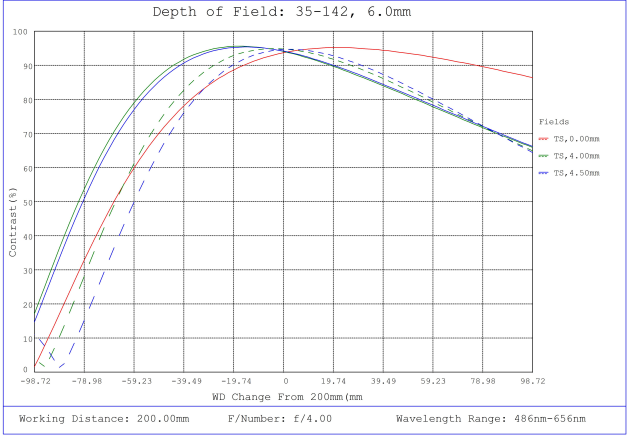
#35-142, 6mm, f/4 Cr Series Fixed Focal Length Lens, Depth of Field Plot, 200mm Working Distance, f4
