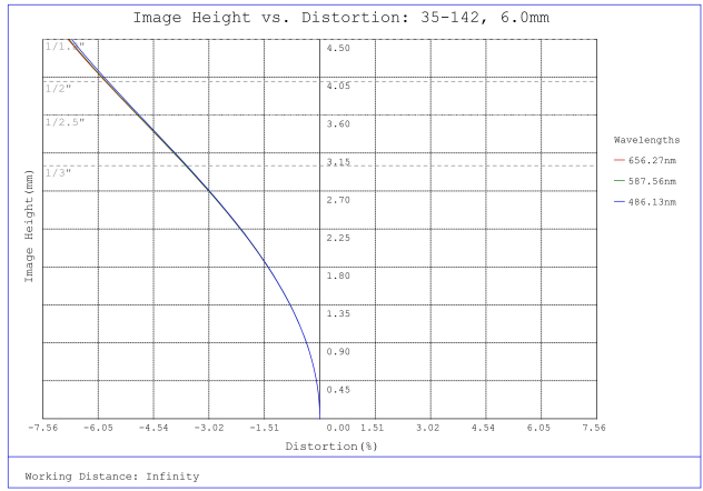
#35-142, 6mm, f/4 Cr Series Fixed Focal Length Lens, Distortion Plot
