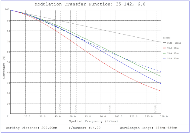
#35-142, 6mm, f/4 Cr Series Fixed Focal Length Lens, Modulated Transfer Function (MTF) Plot, 200mm Working Distance, f4
