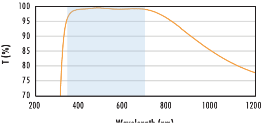
N-BK7 with VIS-EXT Coating Typical Transmission
