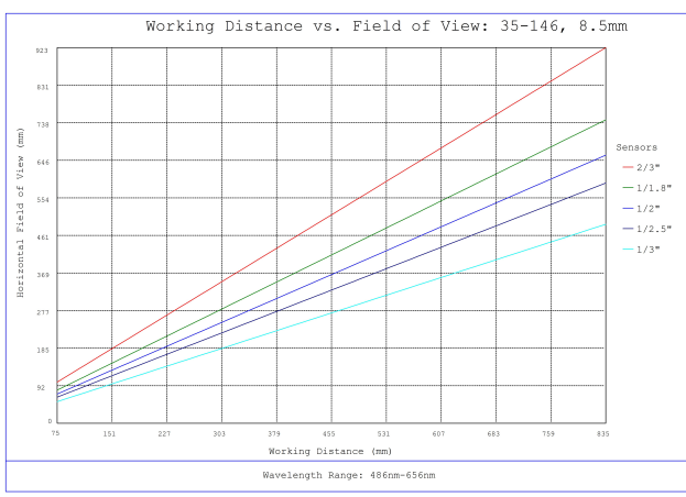
#35-146, 8.5mm, f/1.4, 75mm-∞ Primary WD, HRr Series Fixed Focal Length Lens, Working Distance versus Field of View Plot
