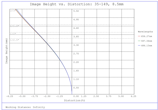
#35-149, 8.5mm, f/2.8, 75mm-∞ Primary WD, HRr Series Fixed Focal Length Lens, Distortion Plot
