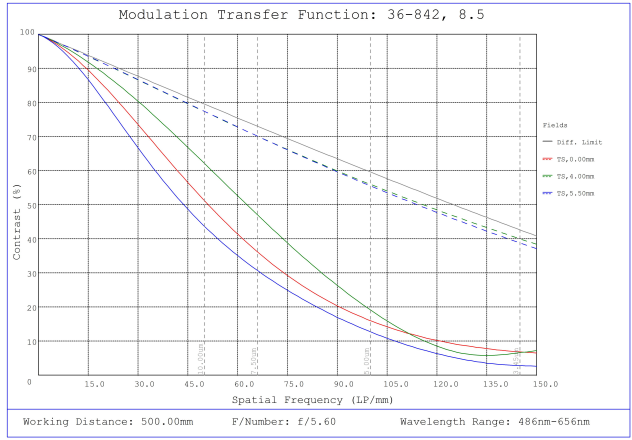
#36-842, 8.5mm, f/5.6 Cr Series Fixed Focal Length Lens, Modulated Transfer Function (MTF) Plot, 500mm Working Distance, f5.6
