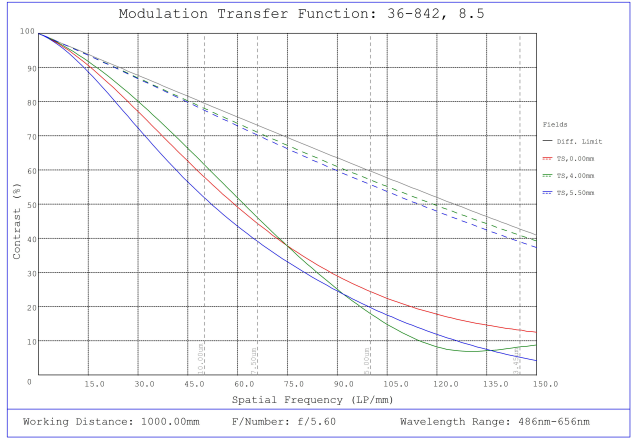
#36-842, 8.5mm, f/5.6 Cr Series Fixed Focal Length Lens, Modulated Transfer Function (MTF) Plot, 1000mm Working Distance, f5.6
