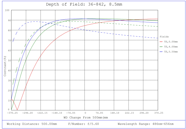
#36-842, 8.5mm, f/5.6 Cr Series Fixed Focal Length Lens, Depth of Field Plot, 500mm Working Distance, f5.6
