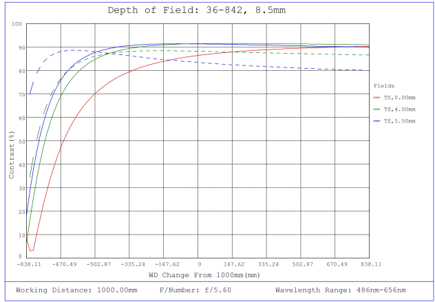
#36-842, 8.5mm, f/5.6 Cr Series Fixed Focal Length Lens, Depth of Field Plot, 1000mm Working Distance, f5.6
