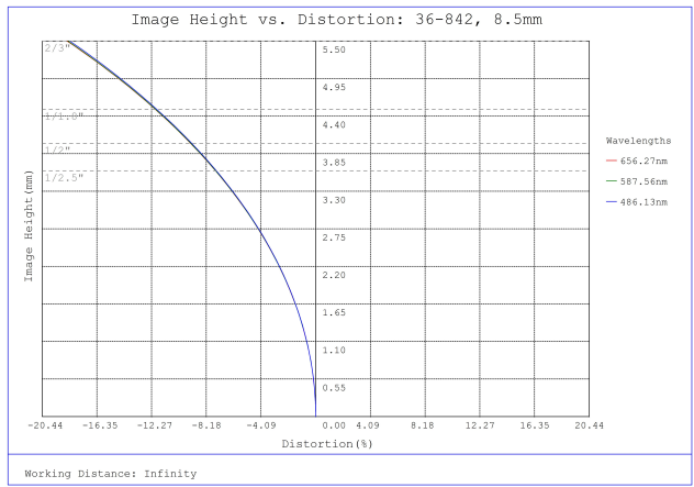
#36-842, 8.5mm, f/5.6 Cr Series Fixed Focal Length Lens, Distortion Plot
