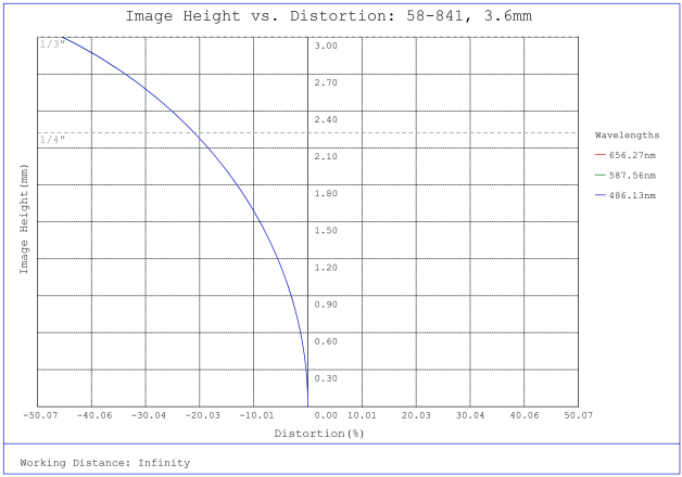
#58-841, f/2.5, Visible, 3.6mm HEO Series M12 Lens, Distortion Plot
