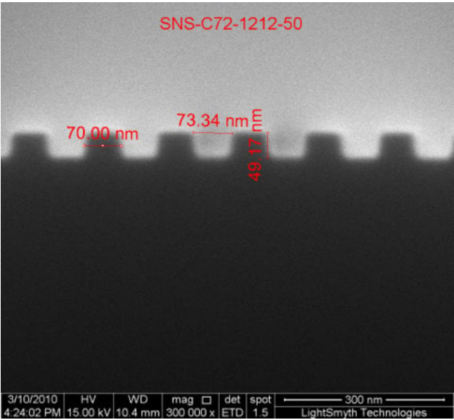
SEM Image of 139nm, 50nm Groove Depth Linear Silicon Nanostamps (Cross Section)
