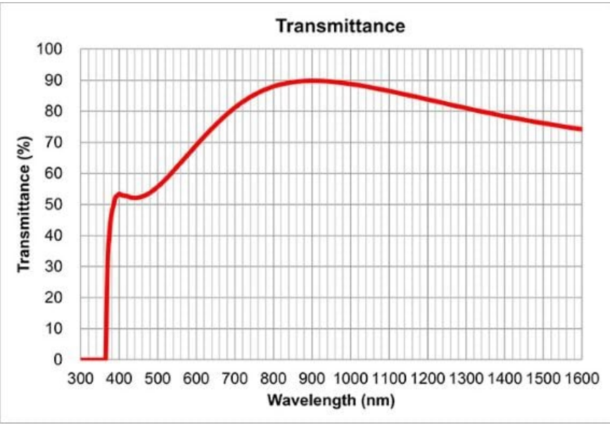
LMPLN10XIR Transmission Graph
