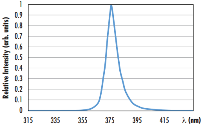
SCHOTT VisiLED Ring Light - UV LED Emission
