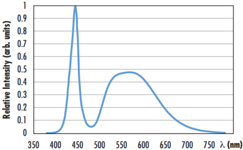
SCHOTT VisiLED Ring Light - White LED Emission
