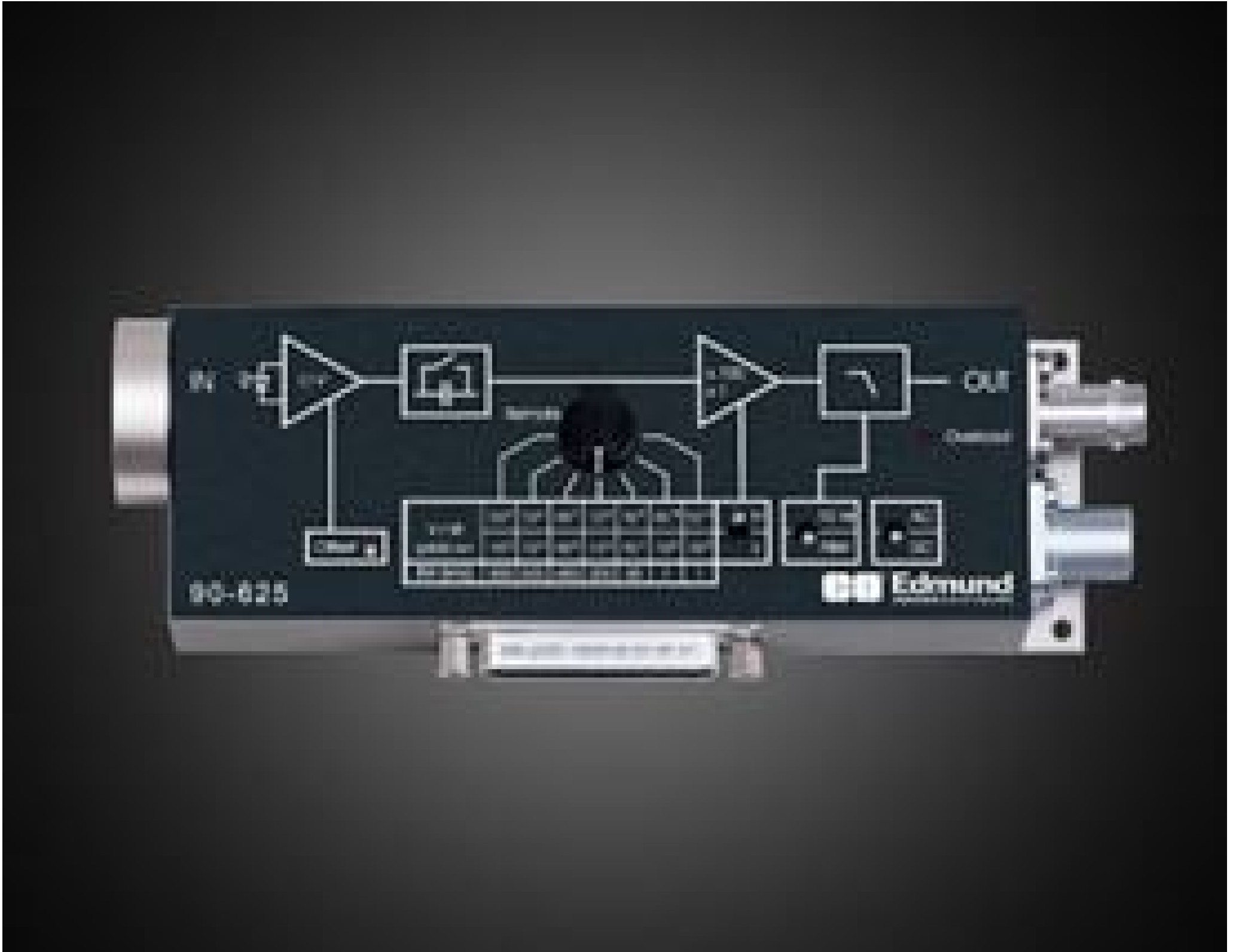
#90-625 SI Variable Gain Photoreceiver, 850nm
